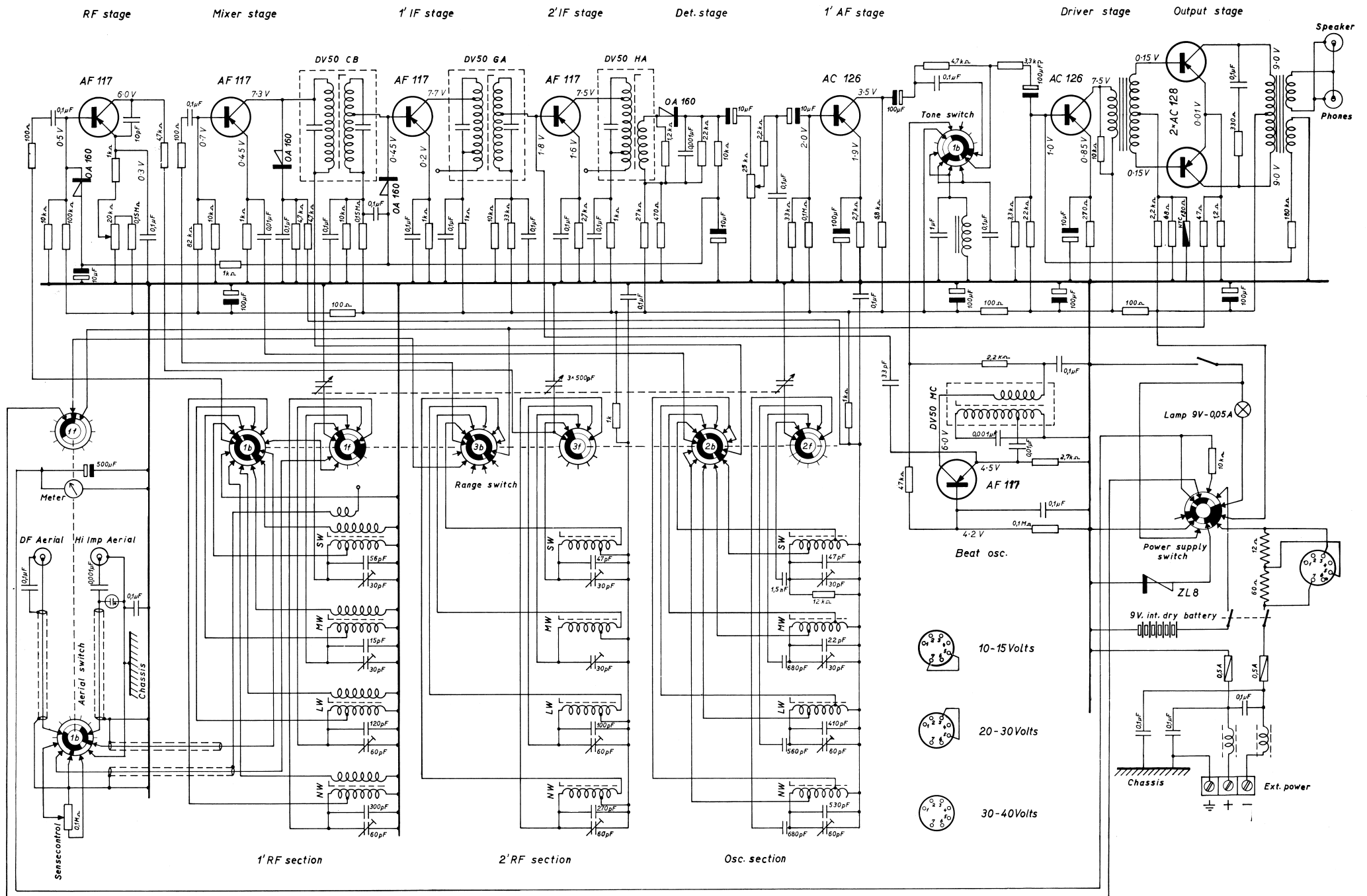
DIAGRAM SAILOR 16 T A/S S. P. RADIO DANMARK
